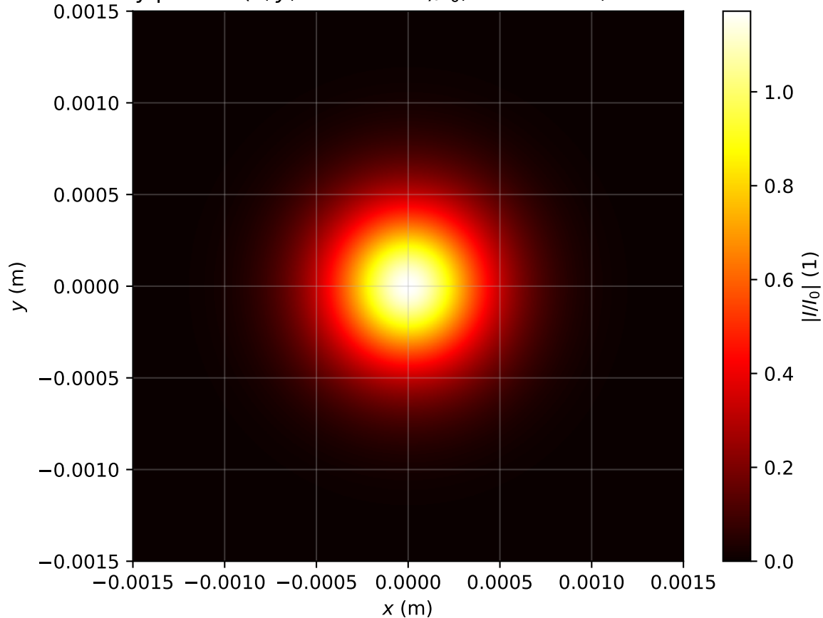
Intensity profile I(x, y, z = 0.637m)/I_0 , Pin=0.8Pcr, artificial time
